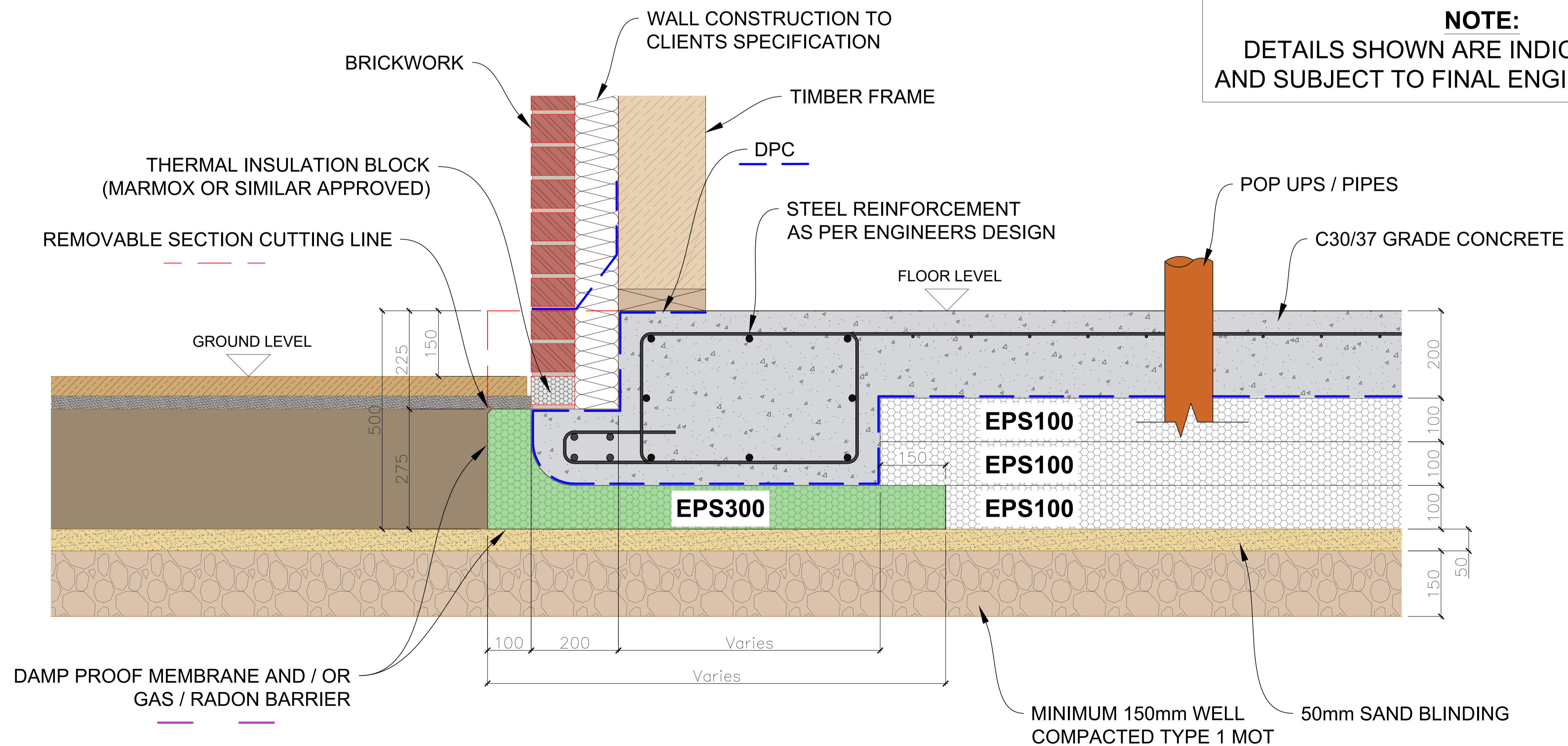
TYPICAL BRICK / TIMBER FRAME EDGE SECTION - AFTER CONCRETE POUR
