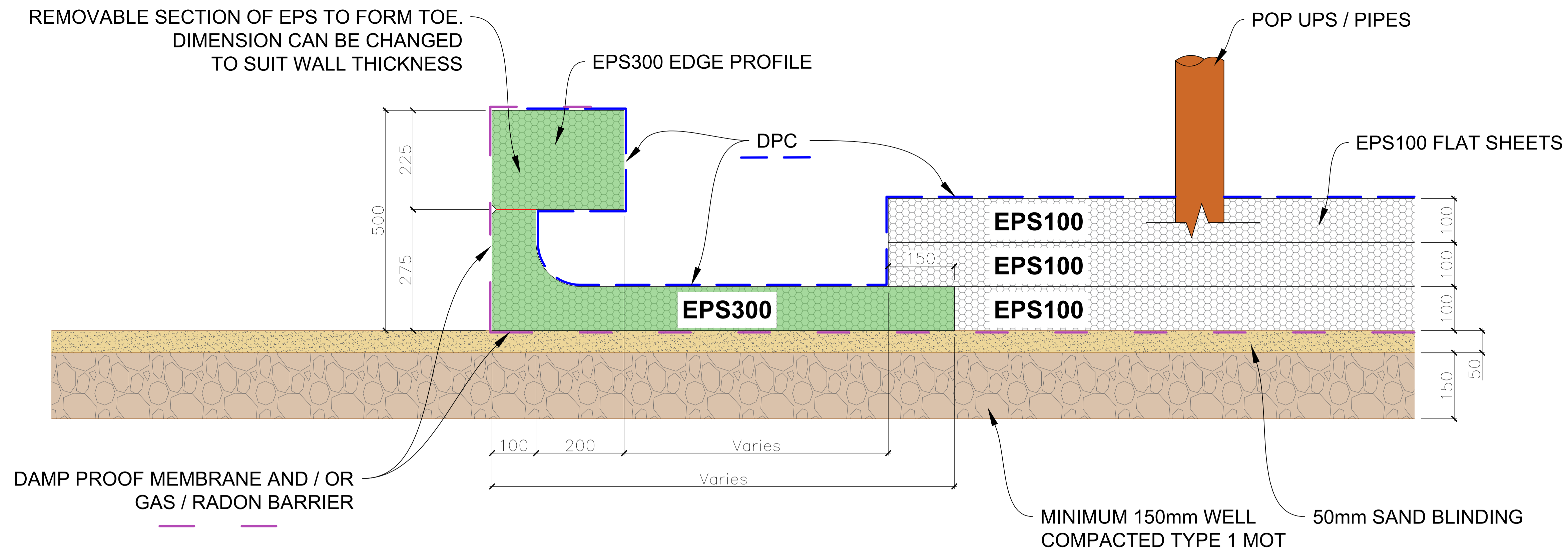
TYPICAL BRICK / TIMBER FRAME EDGE SECTION - BEFORE CONCRETE POUR
