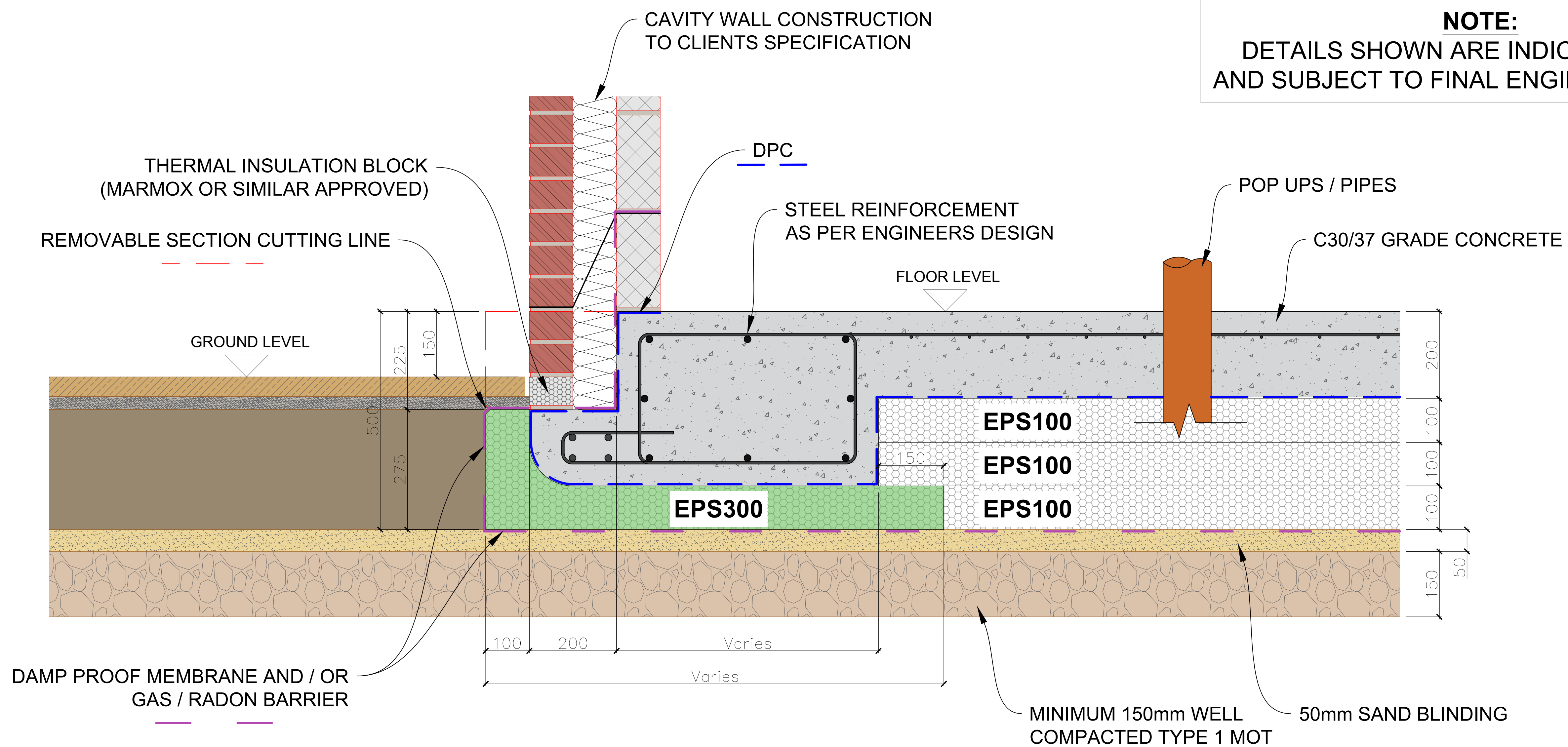
TYPICAL BRICK / BLOCK CAVITY WALL EDGE SECTION - AFTER CONCRETE POUR
