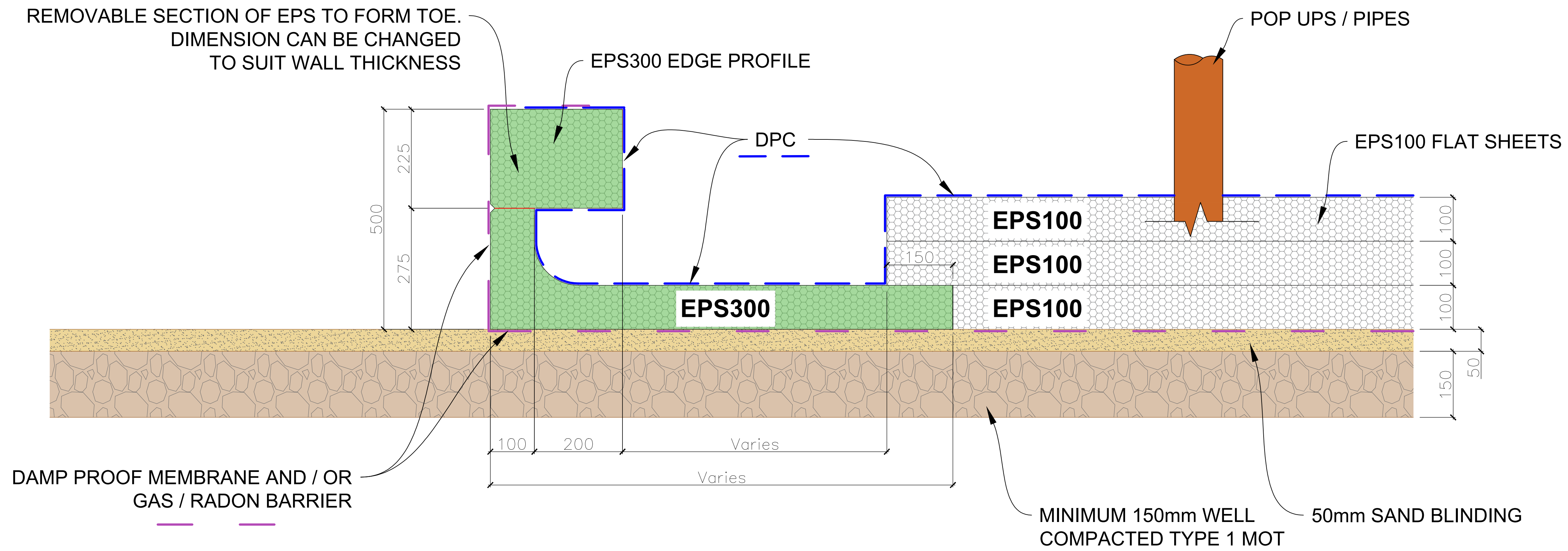
TYPICAL BRICK / BLOCK CAVITY WALL EDGE SECTION - BEFORE CONCRETE POUR
